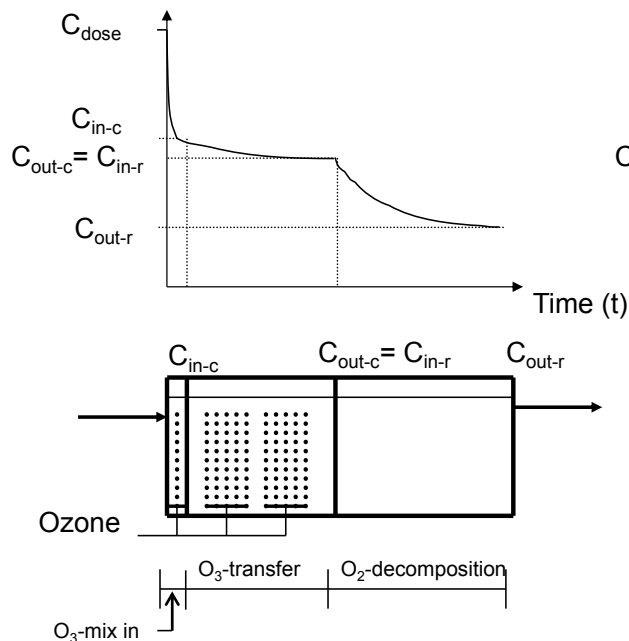
Figure 3.4 Expected progress in concentration change in an ozone transfer system
